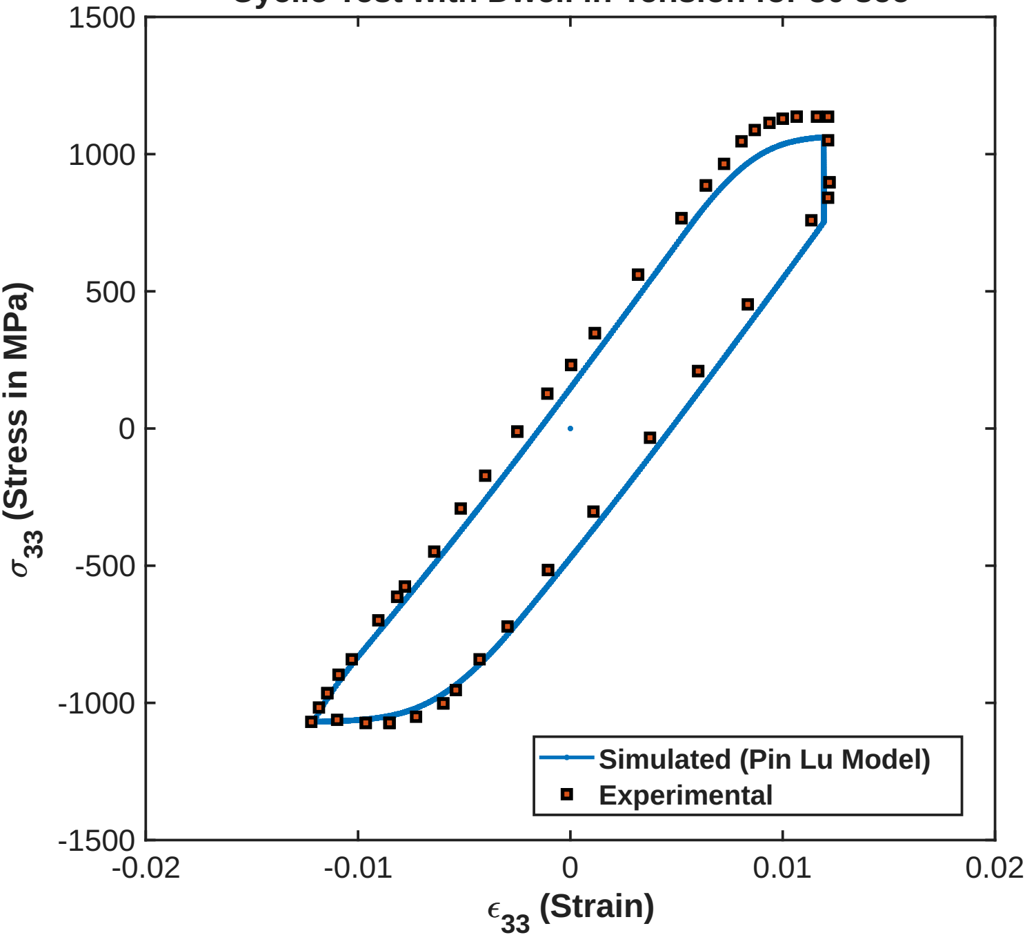
Cyclic Test with Dwell in Tension for 30 sec
